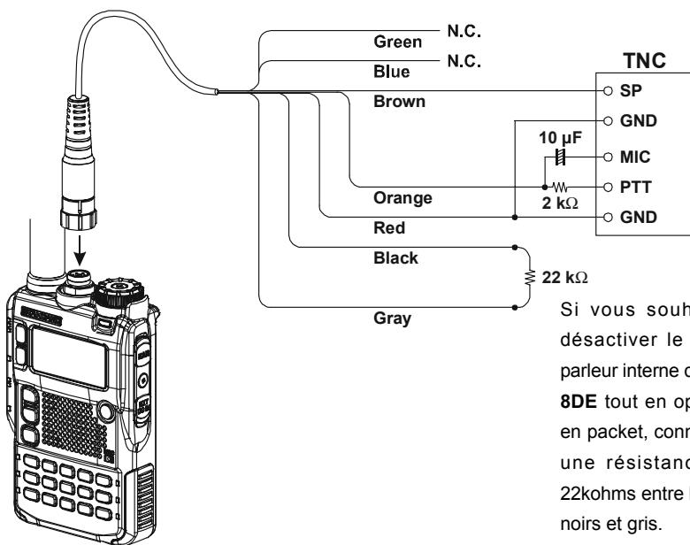
CT-M11 MIC/SP Connection Cable
